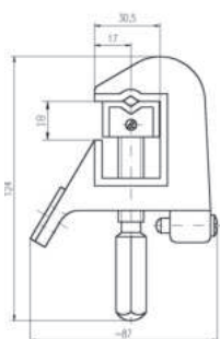
KÖF-C-9001
