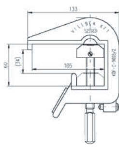
KÖF-C-9003/2
