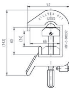
KÖF-C-9002/2
