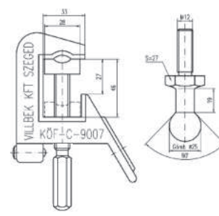
KÖF-C-9007
